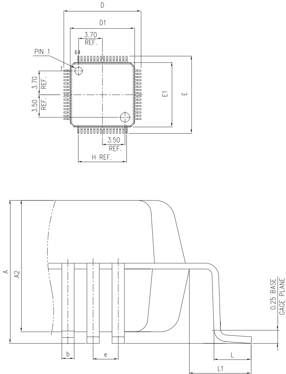
Figure 19 LQFP64 Package Diagram
